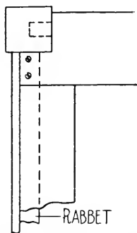
FIG. 395. REINFORCED CORNER FOR TABLES.
